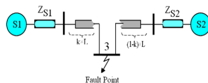
Figure 2. Transmission line during fault.
